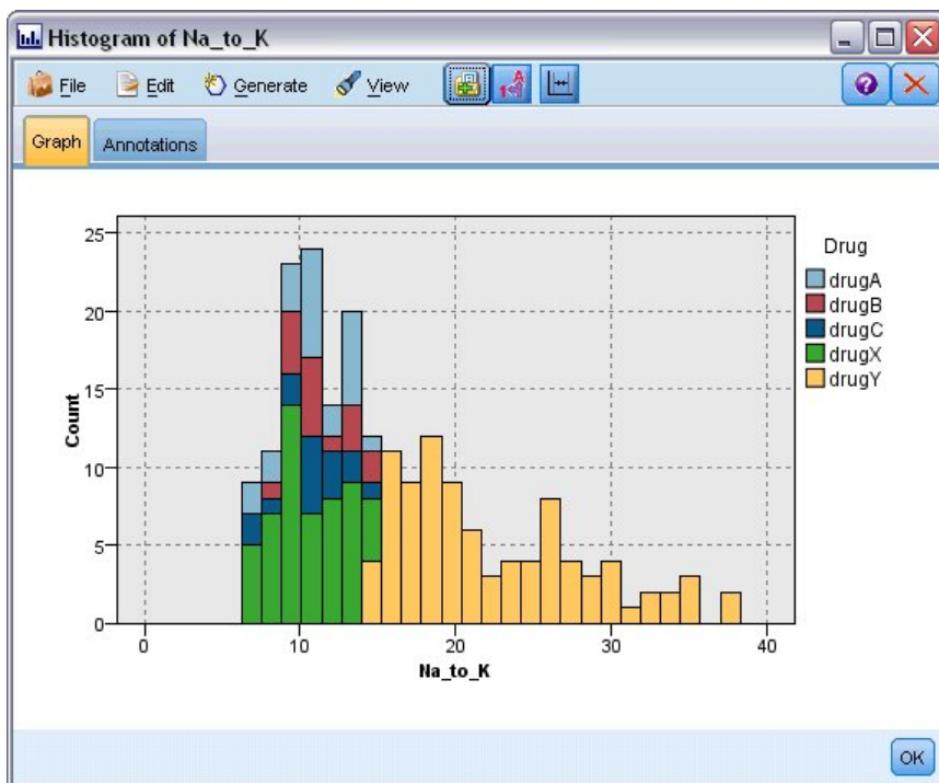
Figure 92. Histogramme
